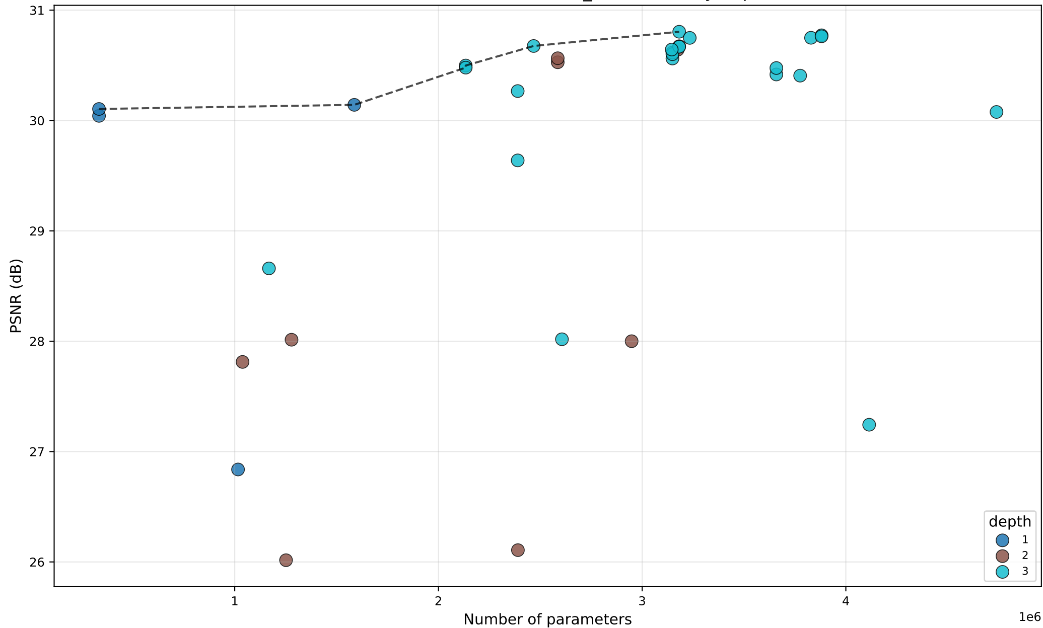
PSNR vs #Params — DHTCUN_baseline — by depth
